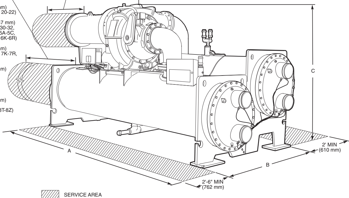
Fig. 7 — 19XR Dimensions (Refer to Tables 1 Through 3)
