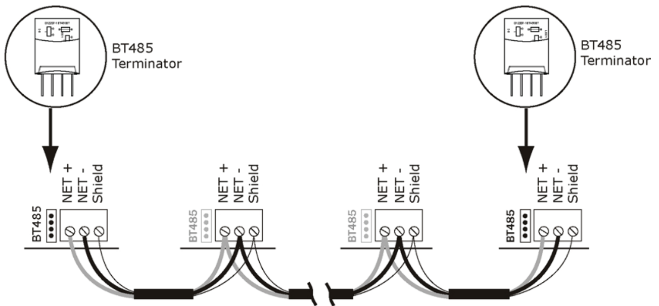
Fig. 40 — Network Wiring
