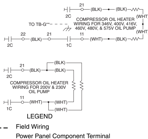
Fig. 38 — Oil Heater and Control Power Wiring (Units with Split Ring Diffuser)
