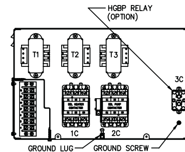
POWER PANEL COMPONENT LAYOUT (SHOWN WITH COVER REMOVED)
