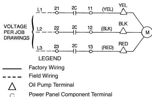
Fig. 36 — Oil Pump Wiring
