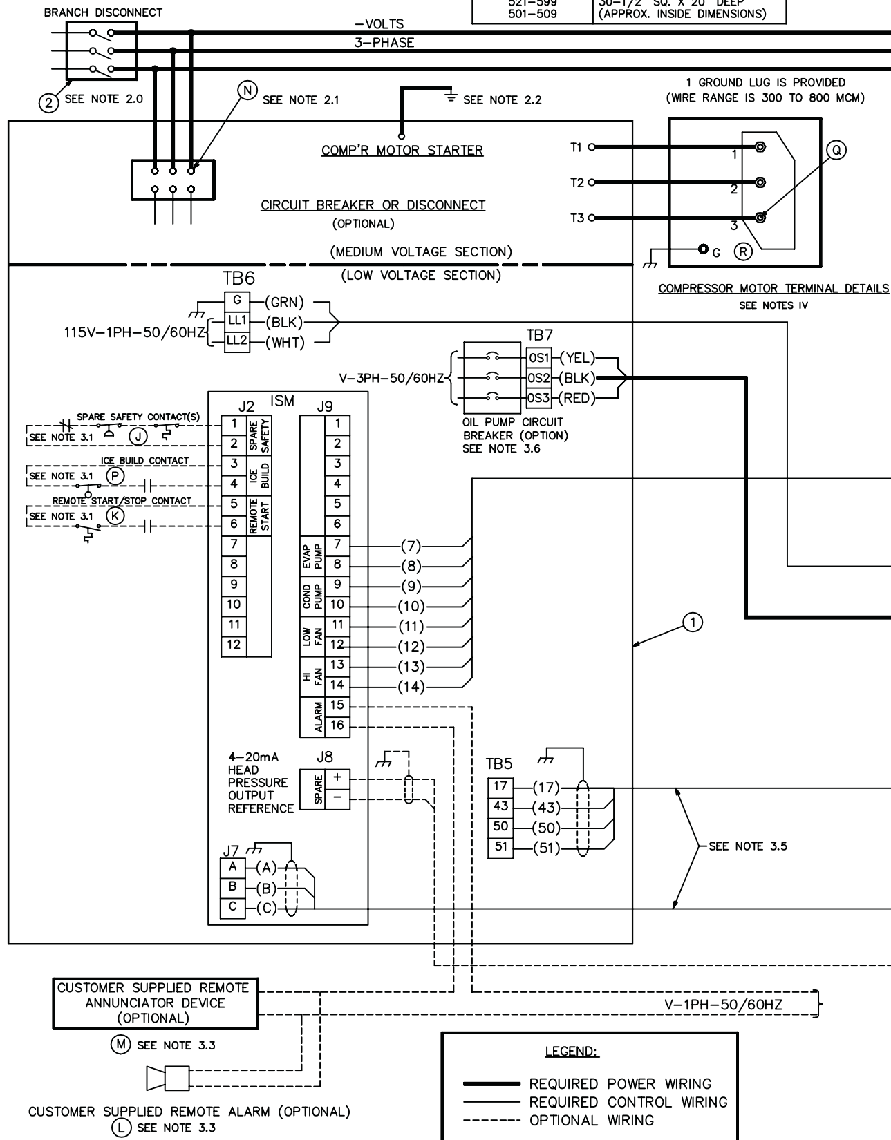
Fig. 34 — 19XR Typical Field Wiring with Free-Standing Starter (Medium Voltage)
