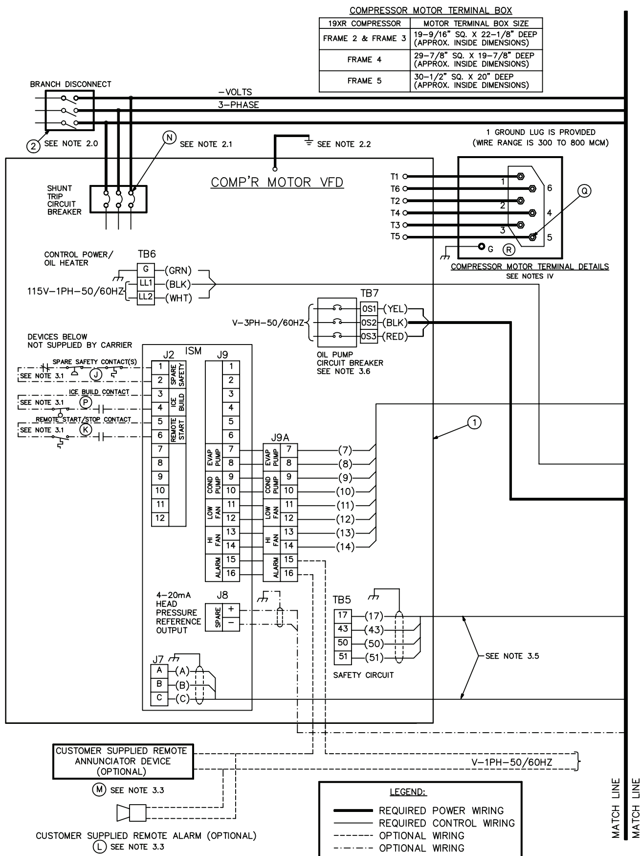
Fig. 35 — 19XR Typical Field Wiring with Free-Standing VFD
