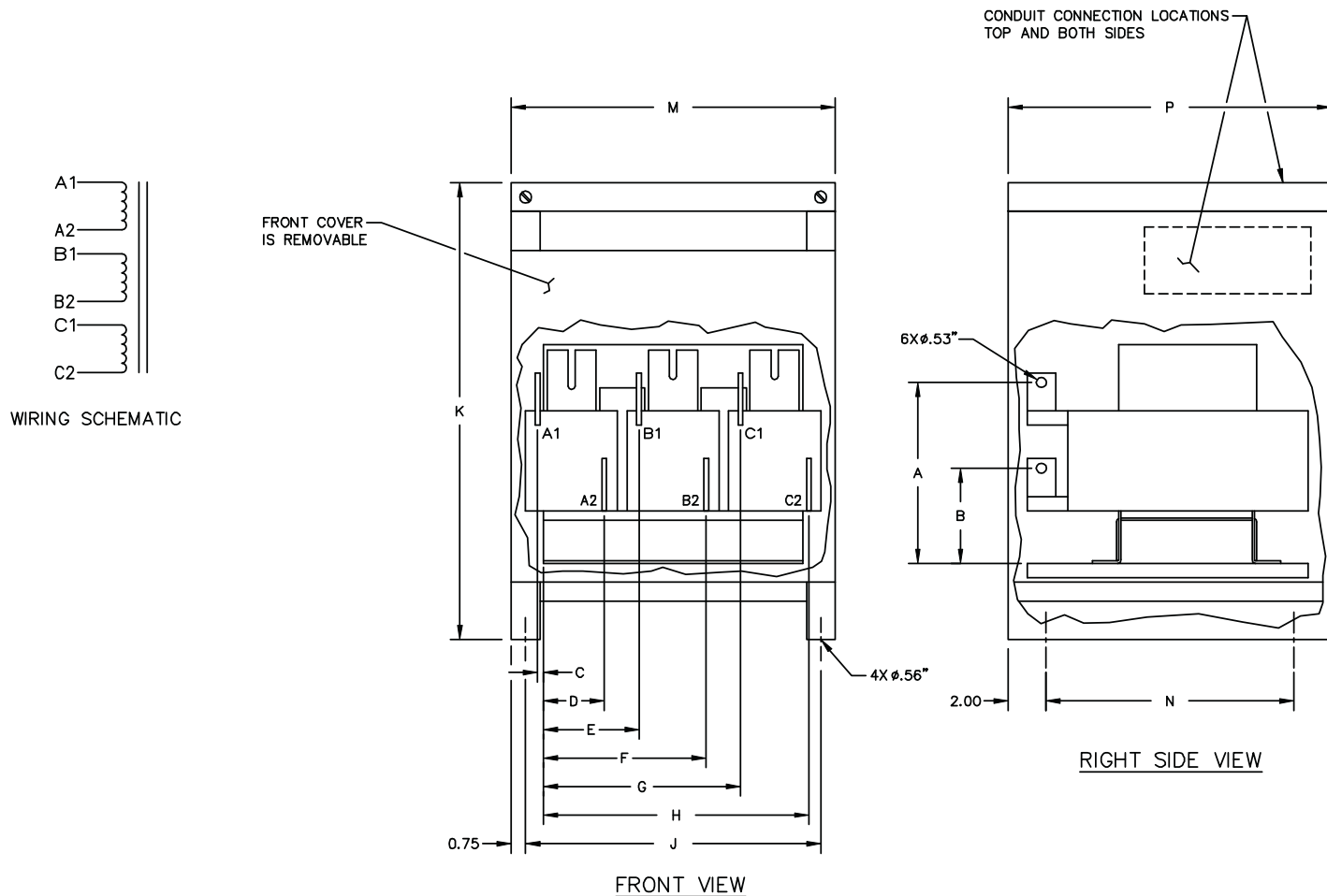
Fig. 31 — 19XRV Optional Line Reactor Physical Dimensions and Field Wiring for Unit-Mounted LF1 VFD Applications
