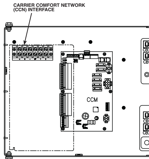
CONTROL PANEL COMPONENT LAYOUT
