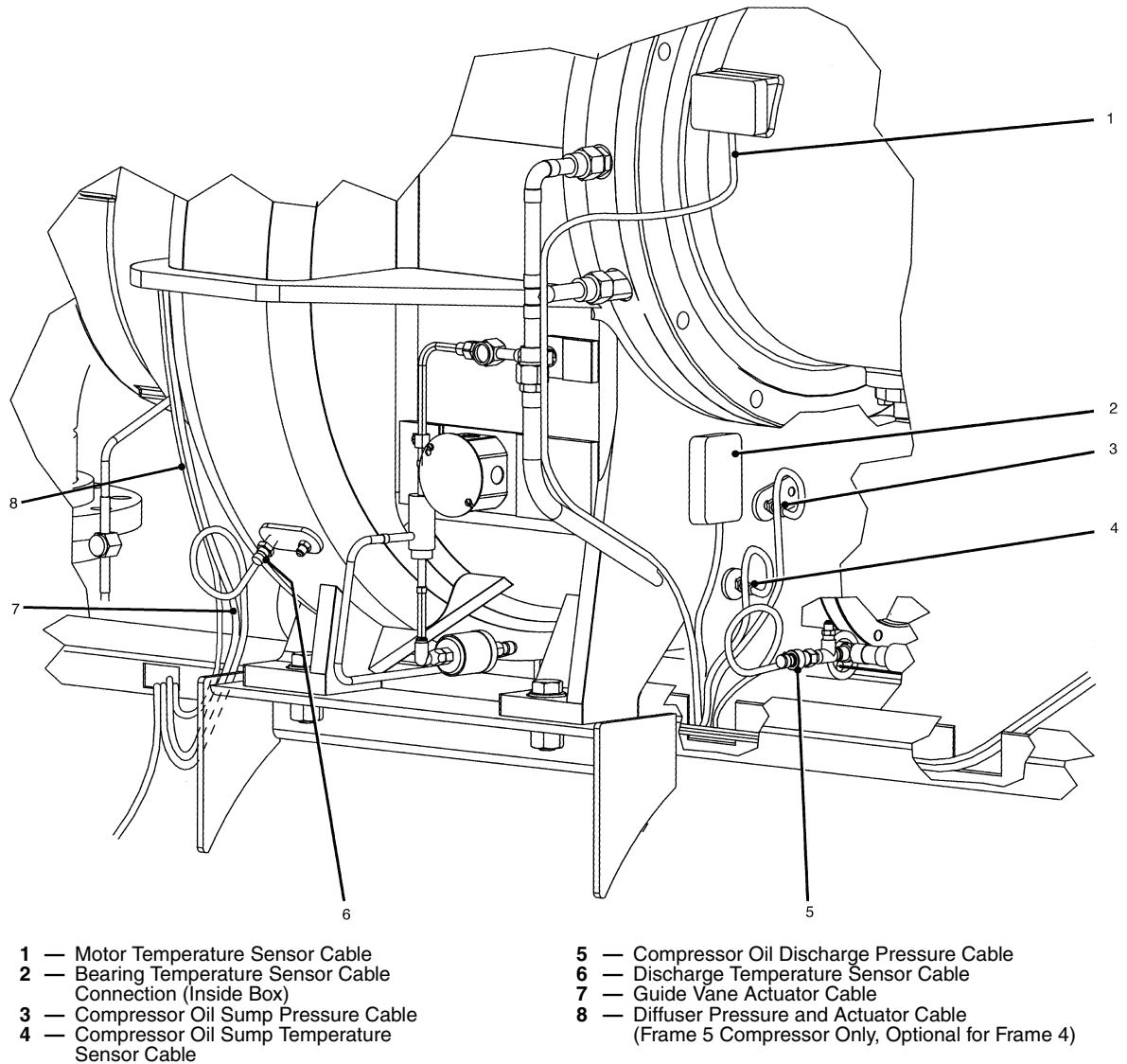
Fig. 10 — Compressor Detail
