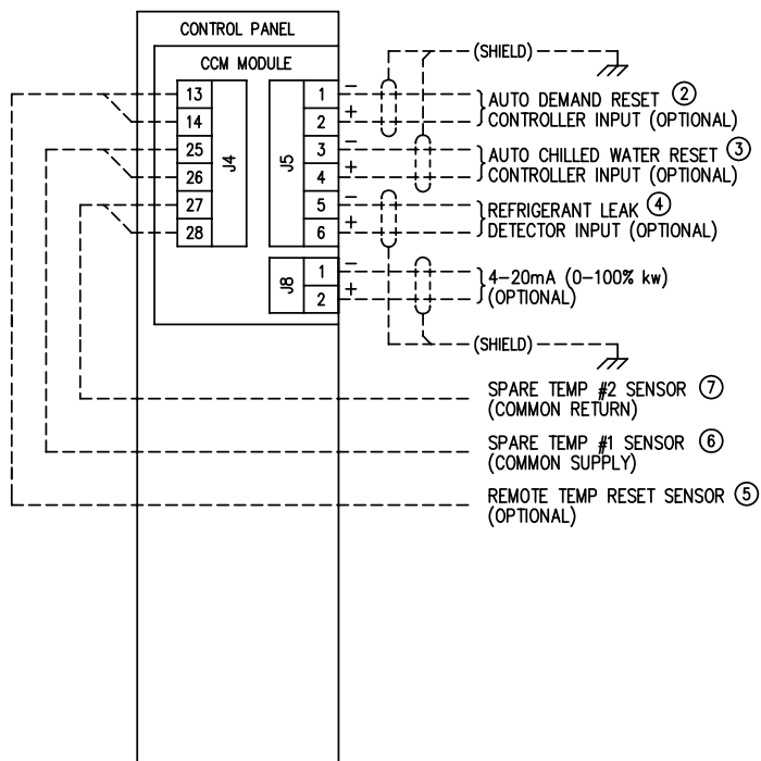
CONTROL PANEL OPTIONAL WIRING
