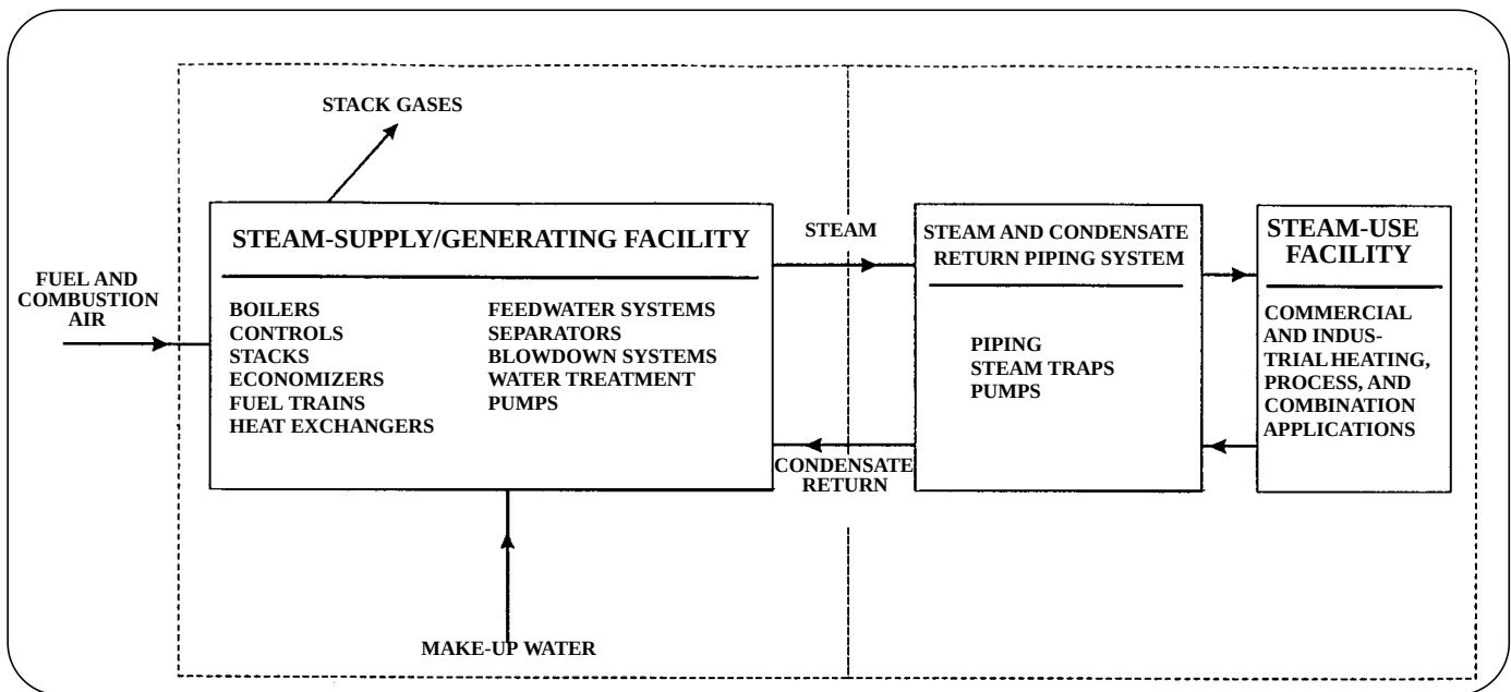
Figure 1. Typical Steam System
