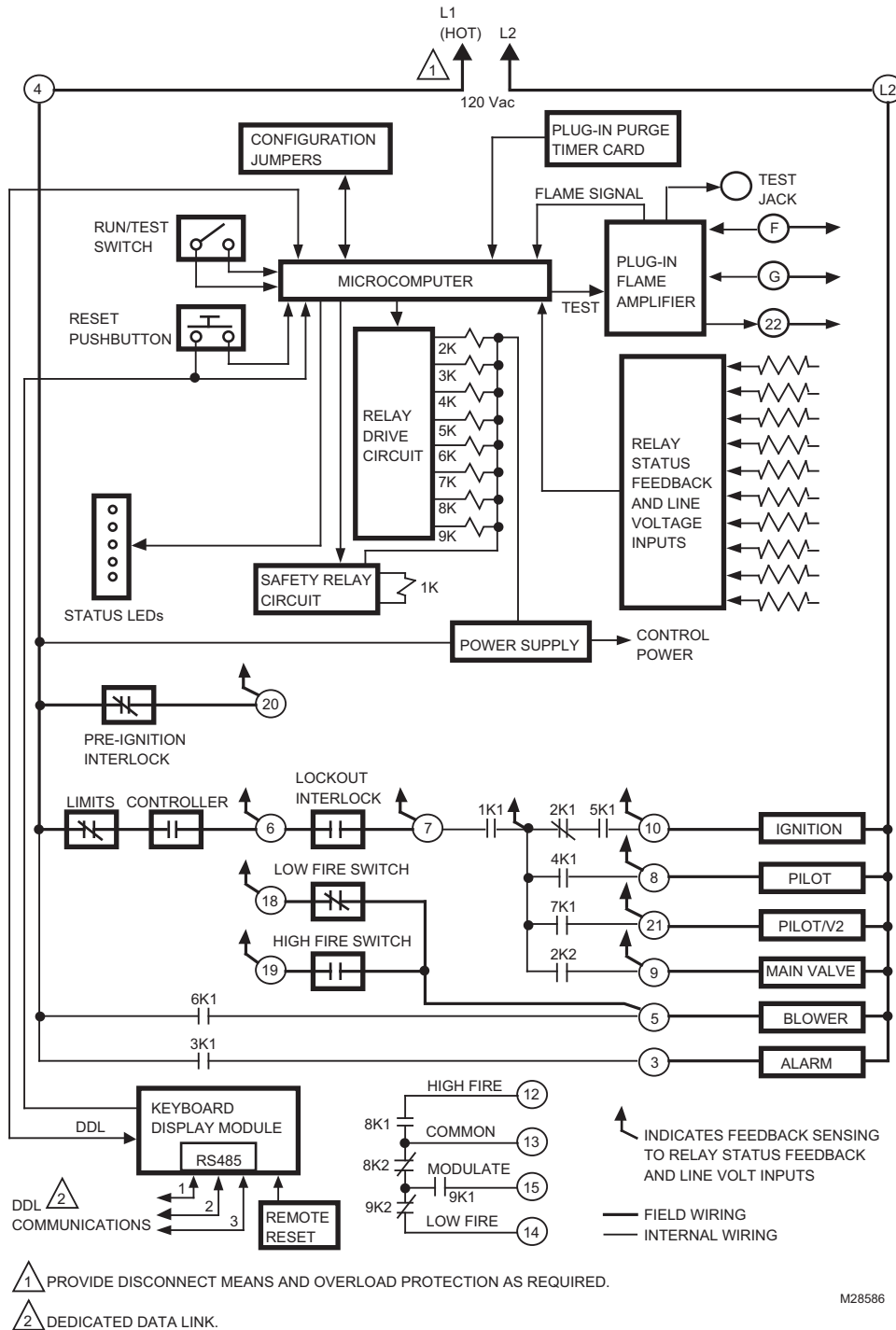
Fig. 7. Internal block diagram of the CB780E/CB784E (see Fig. 8–13 for detailed wiring instructions).
