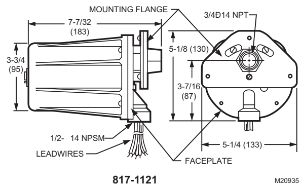
Fig. 4. Ultraviolet Self-Check detector, mounting dimensions in inches (mm).
