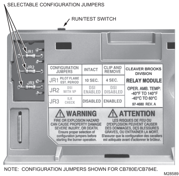
Fig. 39. Selectable site-configurable jumpers.
