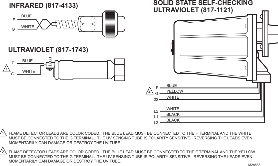
Fig. 20. Flame detector wiring.
