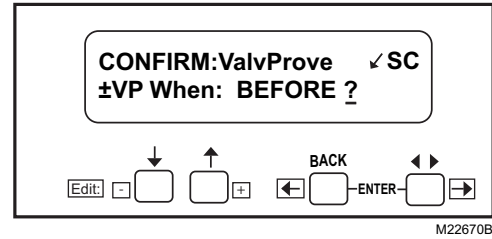
Fig. 31. Confirmation Acknowledgement screen. (The Valve Proving Test location is shown.)
