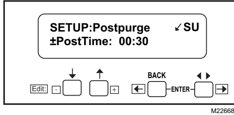
Fig. 29. Setting Postpurge time.
