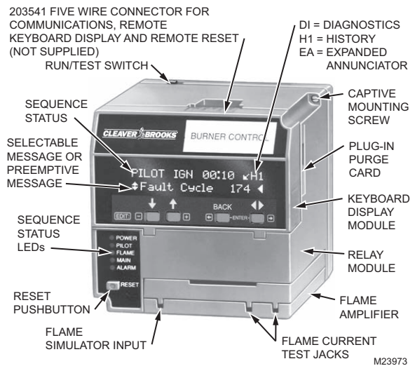
Fig. 40. Keyboard Display Module and sequence status LEDs (Table 4).
