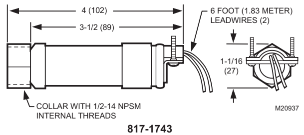
Fig. 5. Ultraviolet detector, mounting dimensions in inches (mm).
