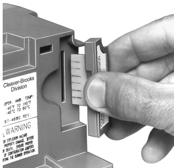
Fig. 15. Purge card installation.
