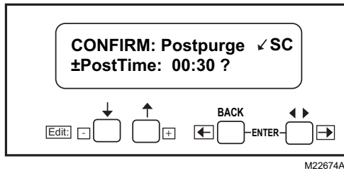
Fig. 35. Confirm Postpurge time.
