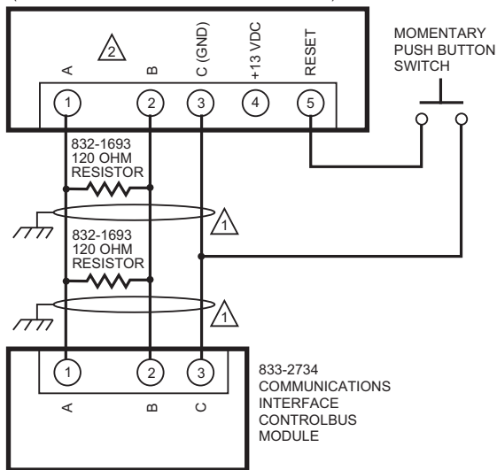
833-2727 KEYBOARD DISPLAY MODULE (MOUNTED ON CB 780/CB 784 RELAY MODULE)
