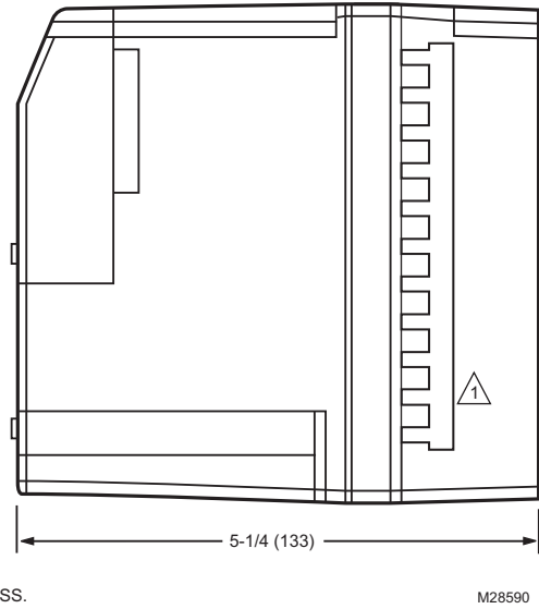
Fig. 2. Mounting dimensions of CB780E/CB784E Relay Module and 833-2725 Subbase, in inches (mm).
