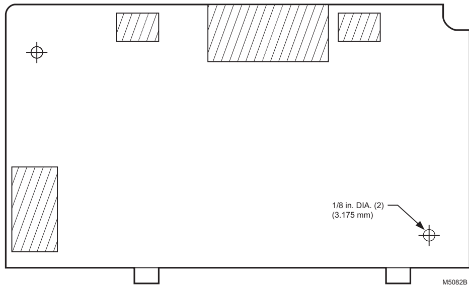
Fig. 50. Flush mounting of a Keyboard Display Module template.
