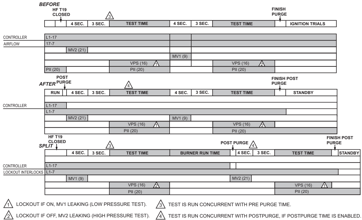
Fig. 10. CB780E/CB784E Relay Module operation, Valve Proving test options.
