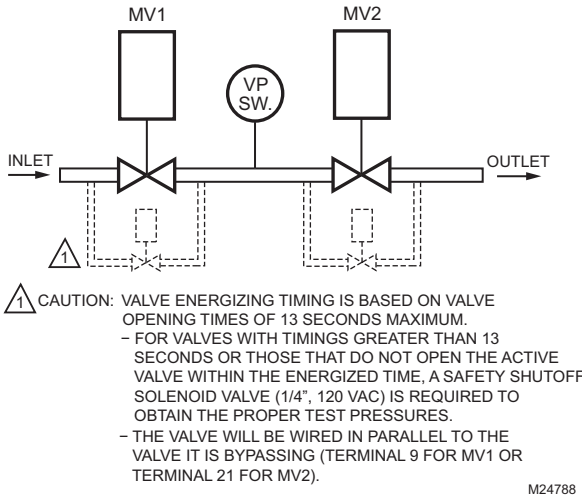
Fig. 1. The valve proving system.
