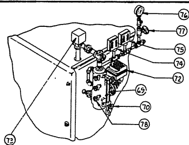
DETAIL FOR LOW WATER CUT OFF LOCATION FRONT CORNER
