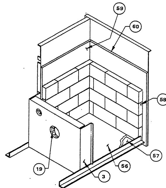
D-450 & D-650 W/BRICKED CHAMBER
