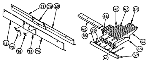
BURNER ASSY. WITH CAST IRON BURNERS (SUPPLIED WITH MOST "CL" BOILERS PRIOR TO JANUARY, 1977)
