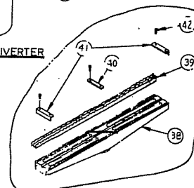
BURNER ASSEMBLY
