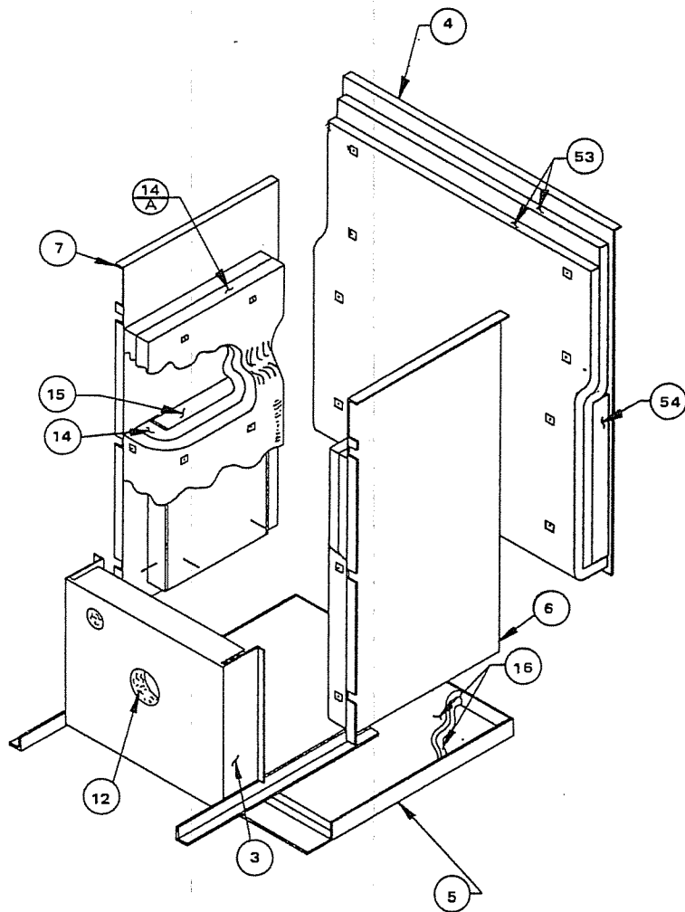
D-650 INSULATION DETAILS
