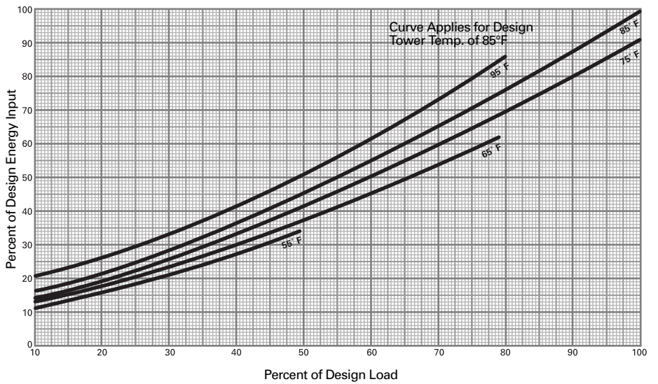
Figure PD-2 — ABSC Part Load Performance – Energy Input vs. Capacity at Various Cooling Water Supply Temperatures; Chilled Water Supply Temperature = 44°F (7°C) (Fixed Chilled Water Flow) with Economizer
