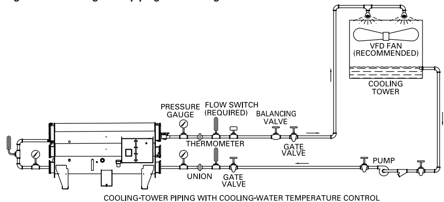
Figure JC-5. Cooling-water piping with cooling tower
