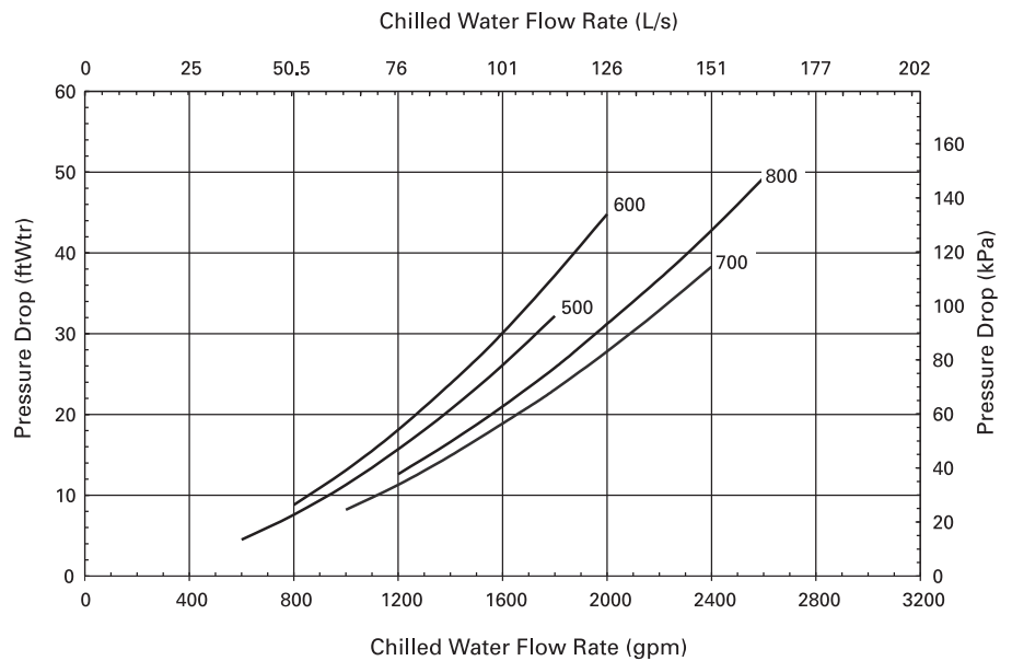
Figure PD-5. ABSD 500-800 pressure drop vs. chilled water flow rate – English and SI Units
