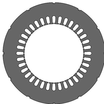
Stator Lamination
