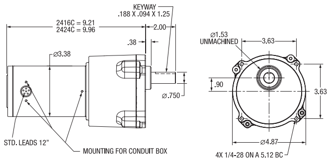
1. 24 - PSL 3 & 4 STAGES
