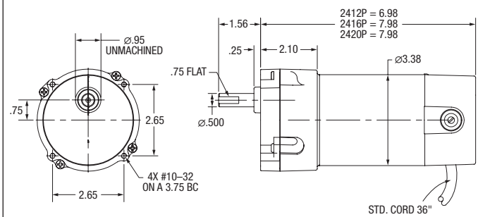
3. 24 - PSSH 3 & 2 STAGES
