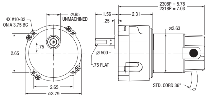
2. 23 - PSSH 3 & 2 STAGES
