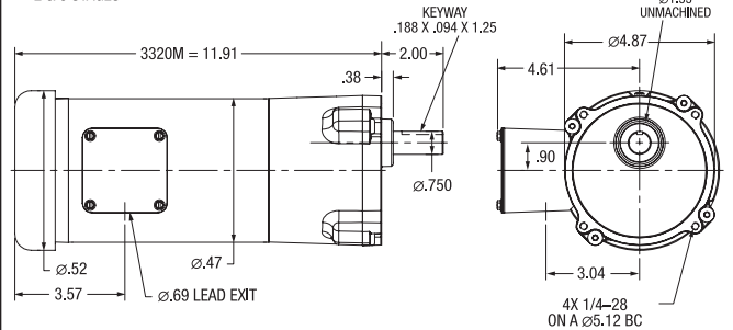
6. 33 - PSLH 2 & 3 STAGES
