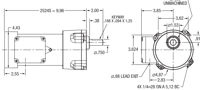
3. 25 - PSL 2 STAGES
