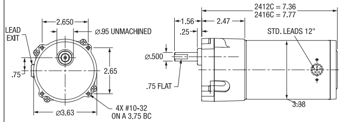
2. 24 - PSSH 4 & 5 STAGES
