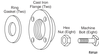
Companion Flange Kit
