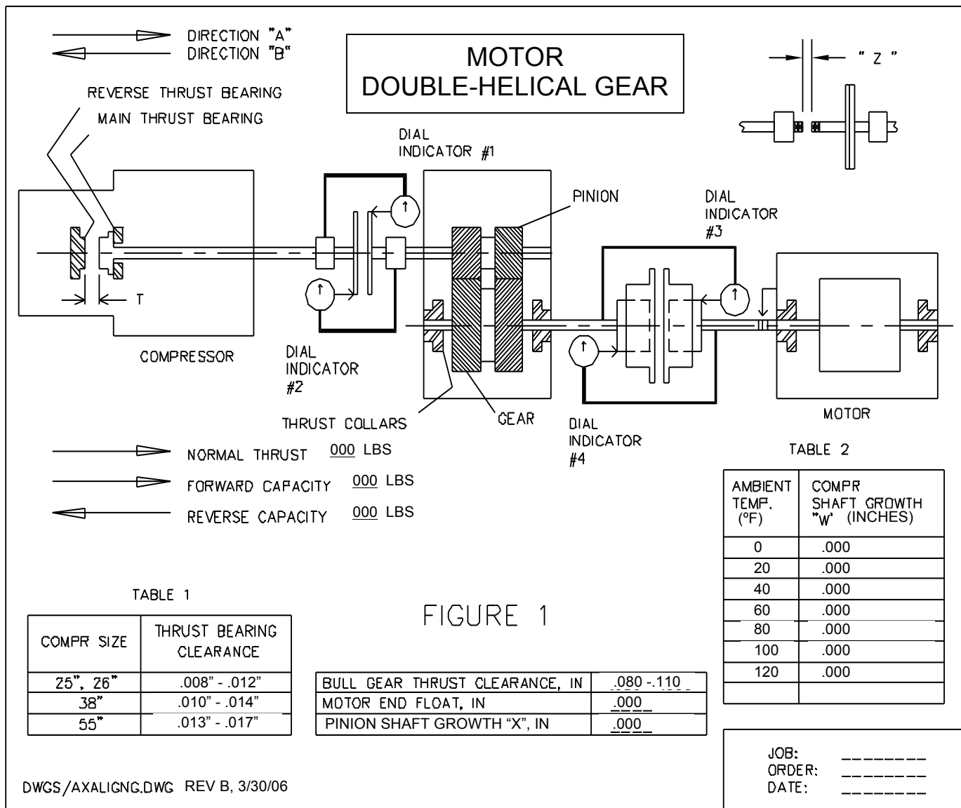
Axial Alignment Drawing
