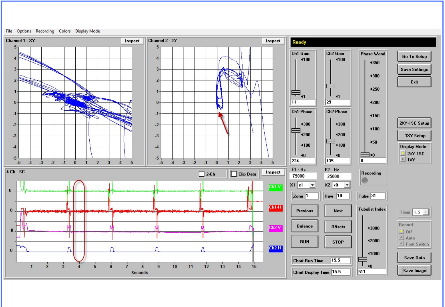
ID PIT 40% - 59% (Row 10 Tube 31)
