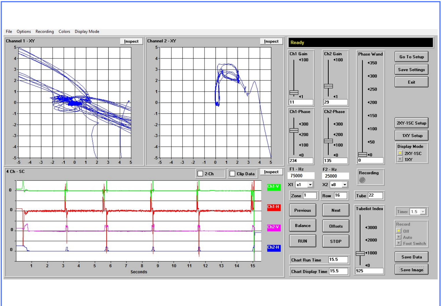
DIFFERENT TUBE TYPE (Row 14 Tube 22)
