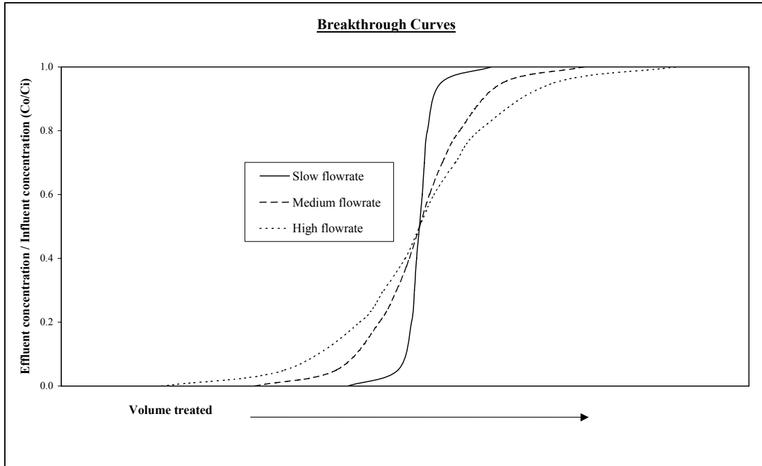
Figure 1.4: Breakthrough curve showing the outlet concentration.
