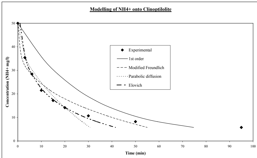
Figure 7.4: Kinetic models of NH 4 + onto clinoptilolite.
