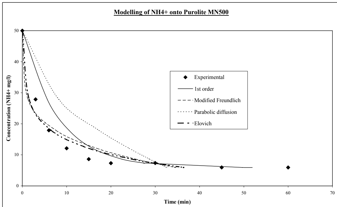
Figure 7.5: Kinetic models of NH 4 + onto Purolite MN500.
