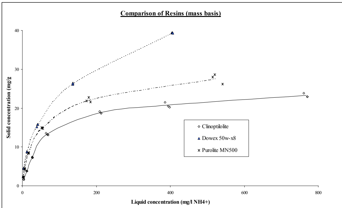
Figure 4.20: NH 4 + equilibrium for each ion exchange resin (mass basis).
