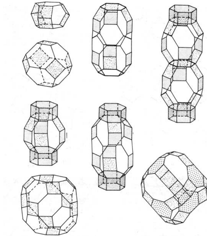
Figure 1.7: Various zeolitic structures [14] .
