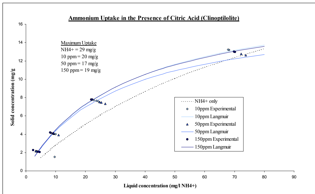
Figure 4.8: NH 4 + equilibrium in the presence of citric acid, onto clinoptilolite.
