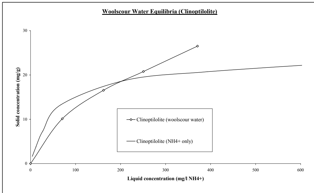
Figure 4.22: NH 4 + equilibrium of woolsour water onto clinoptilolite.
