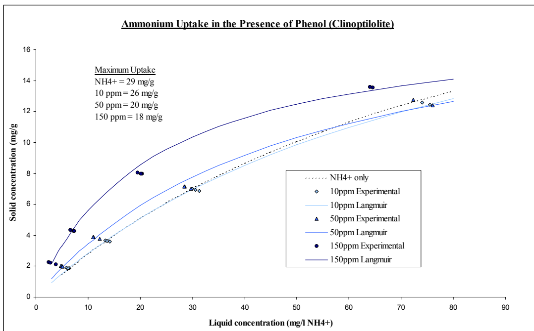
Figure 4.5: NH 4 + equilibrium in the presence of phenol, onto clinoptilolite.
