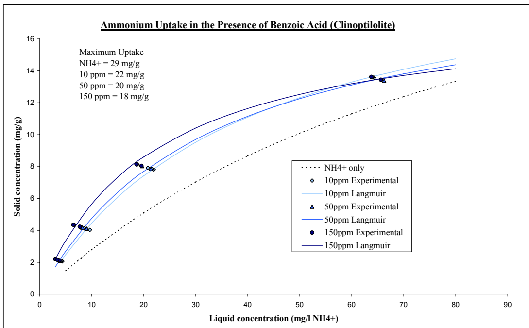
Figure 4.3: NH 4 + equilibrium in the presence of benzoic acid, onto clinoptilolite.
