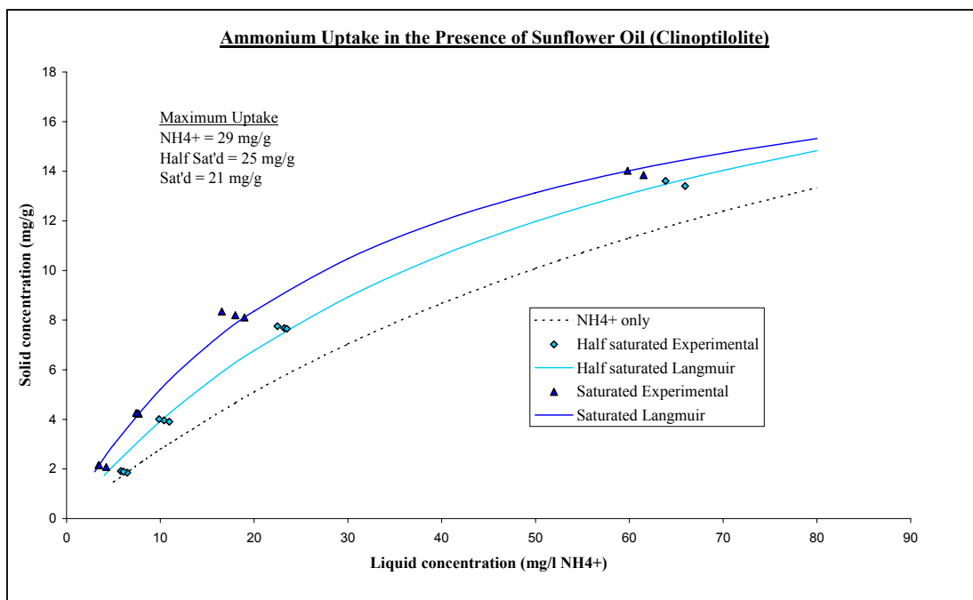
Figure 4.12: NH 4 + equilibrium in the presence of sunflower oil, onto clinoptilolite.
