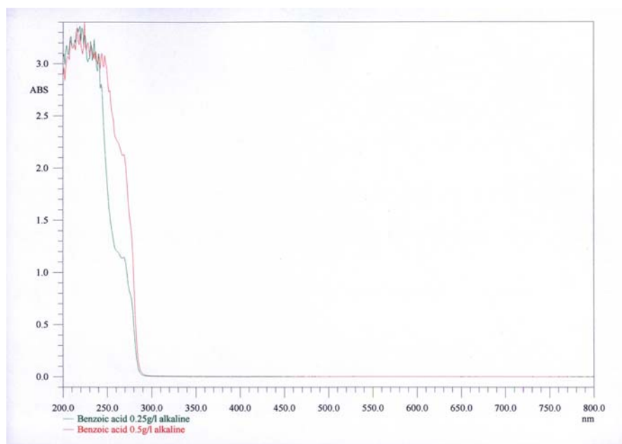
UV/vis (190nm – 800nm) absorption of benzoic acid at pH = 11.0 at two different concentrations.
