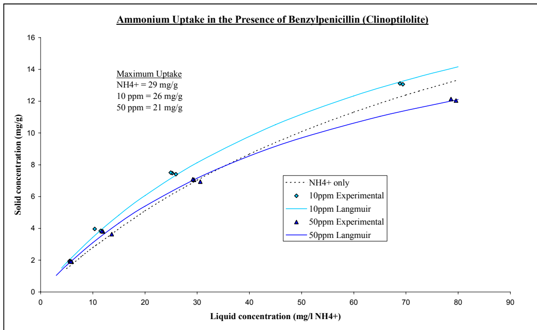
Figure 4.11: NH 4 + equilibrium in the presence of benzylpenicillin G potassium salt, onto clinoptilolite.
