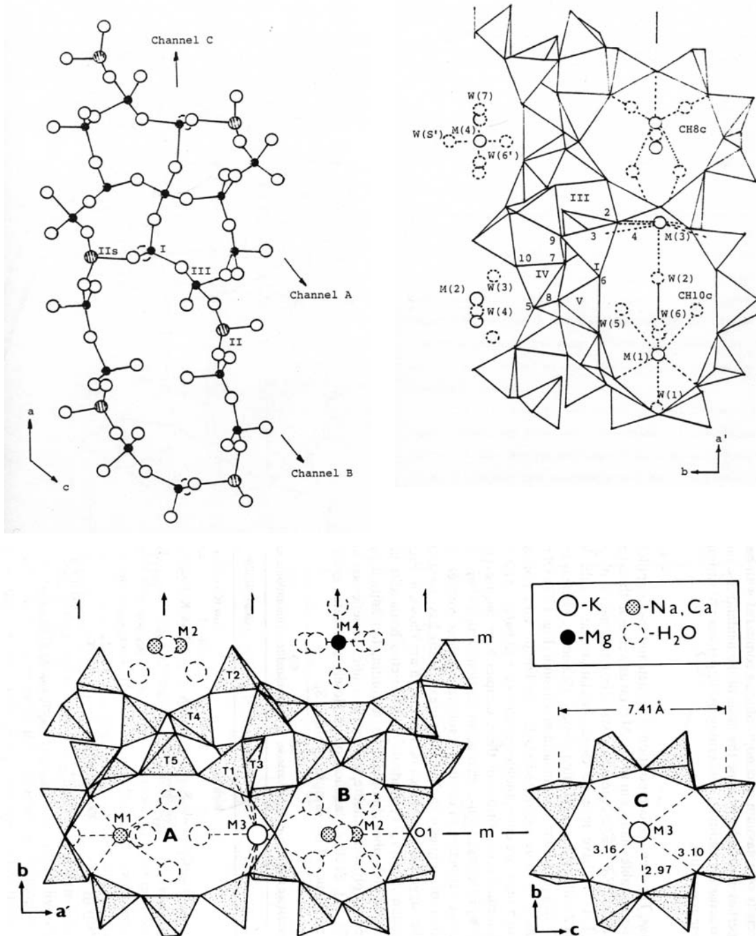
Figure 1.10: Crystalline structure of clinoptililite. [14,16]
