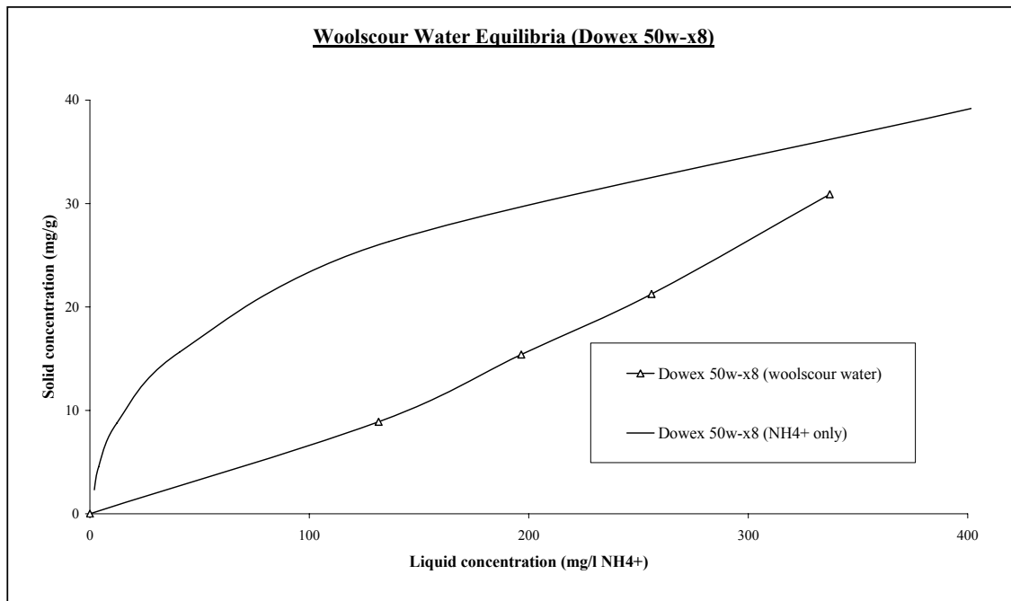
Figure 4.23: NH 4 + equilibrium of woolscour water onto Dowex 50w-x8.
