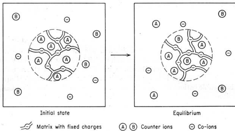
Figure 1.3: Ion exchange equilibrium [1] .
