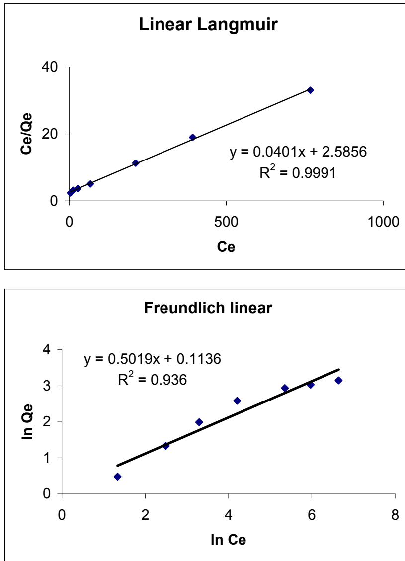
Linear forms of the Langmuir and Freundlich models onto clinoptilolite (figure 4.1).
