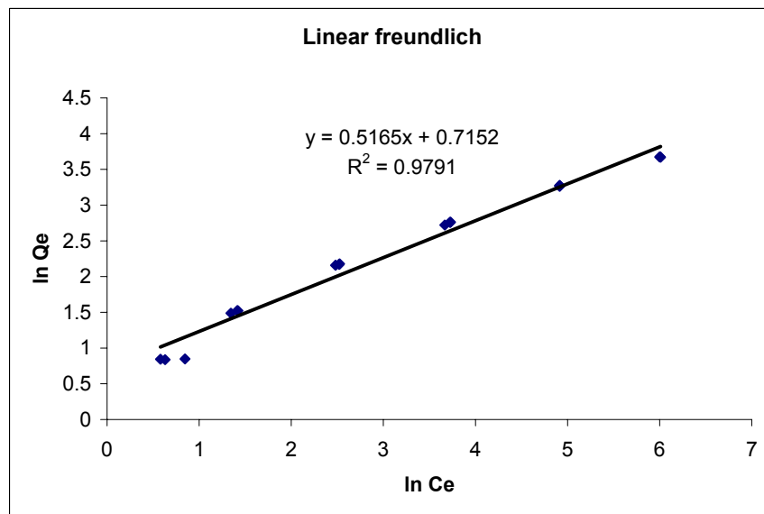
Linear forms of the Langmuir and Freundlich models onto Dowex 50w-x8 (figure 4.14).
