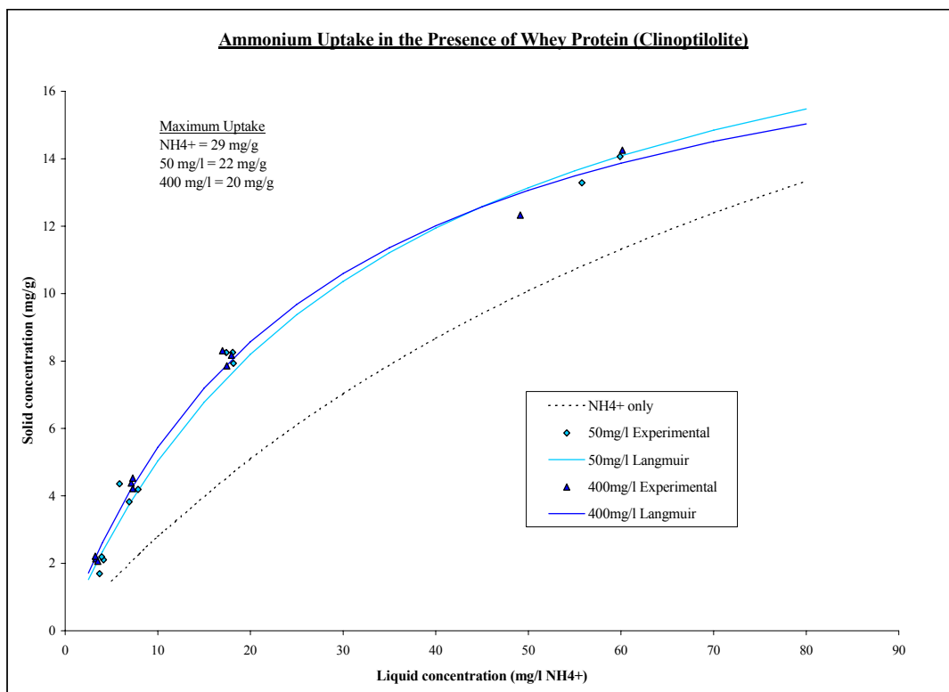
Figure 4.13: NH 4 + equilibrium in the presence of whey protein, onto clinoptilolite.
