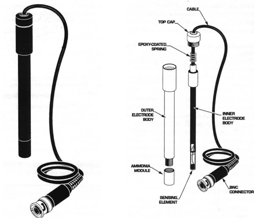
Figure 3.1: Hach 50250 & Orion 95-12 ammonia ion selective electrode.
