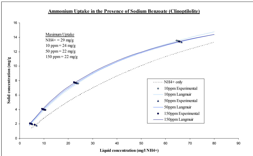
Figure 4.4: NH 4 + equilibrium in the presence of sodium benzoate, onto clinoptilolite.
