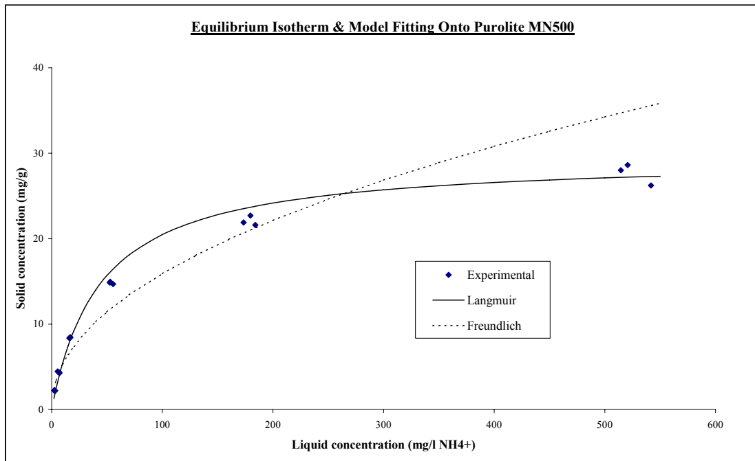
Figure 4.17: Equilibrium of \text{NH}_4^+ onto Purolite MN500.
