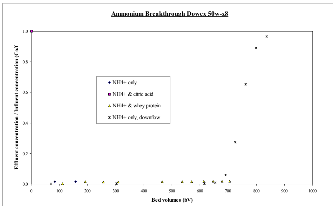
Figure 6.14: Ammonium ion breakthrough in a column of Dowex 50w-x8.
