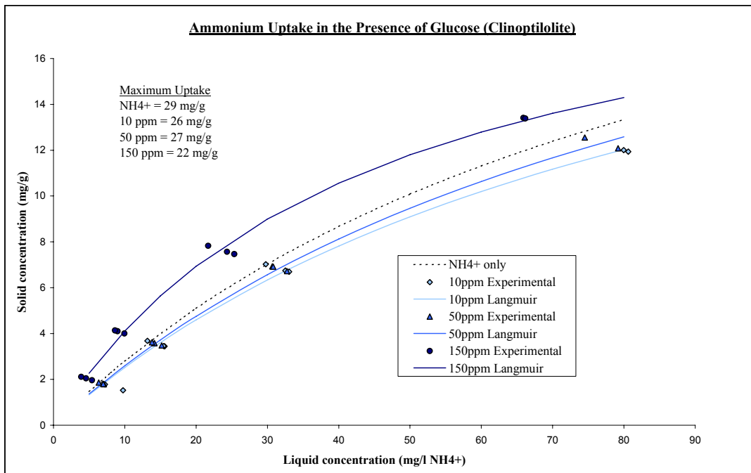
Figure 4.7: NH 4 + equilibrium in the presence of glucose, onto clinoptilolite.
