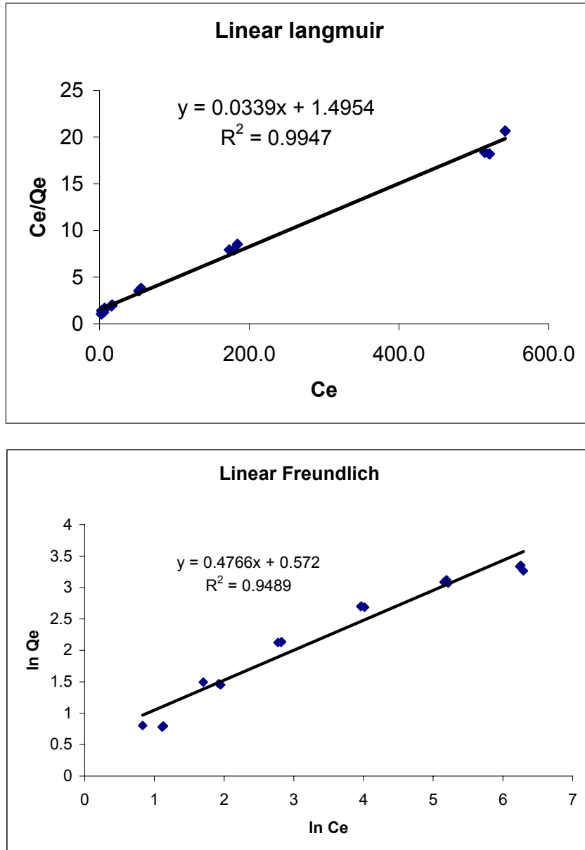
Linear forms of the Langmuir and Freundlich models onto Purolite MN500 (figure 4.17).
