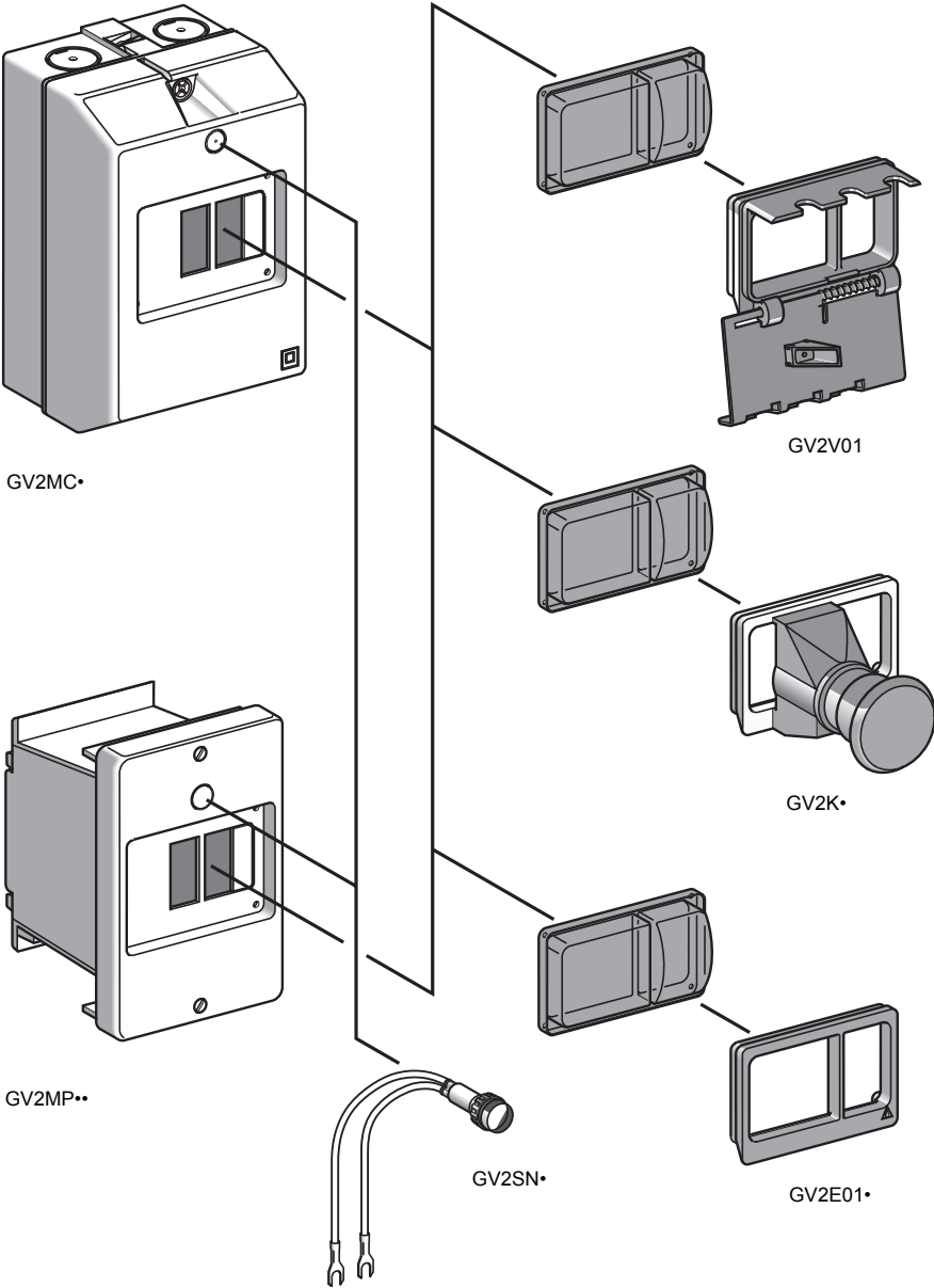
Figure 4: GV2M Enclosures
