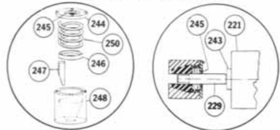
Segmented Bearing Detail
