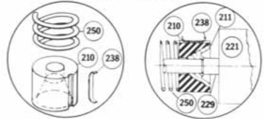
Conical Bearing Detail
