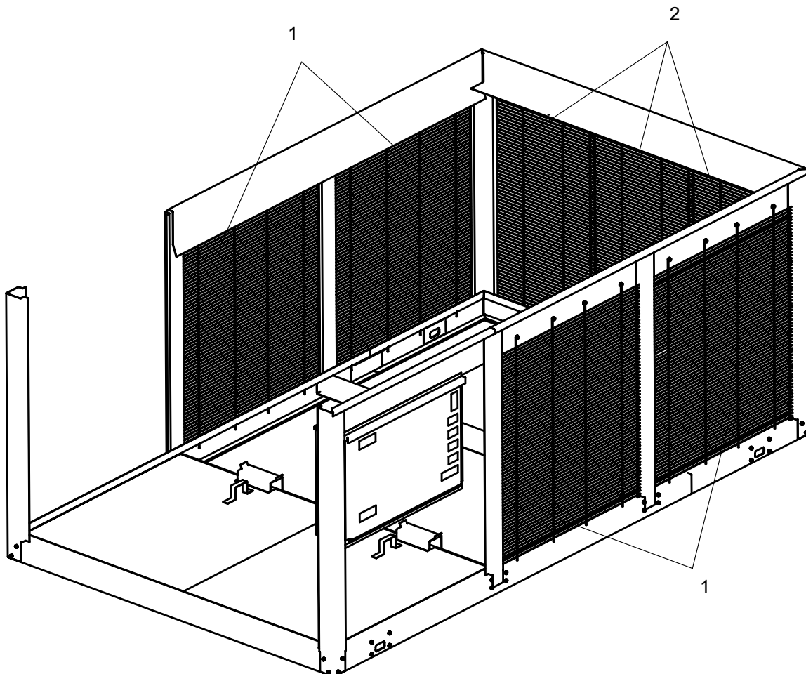
FIGURE 24 - WIRE ENCLOSURE PARTS
