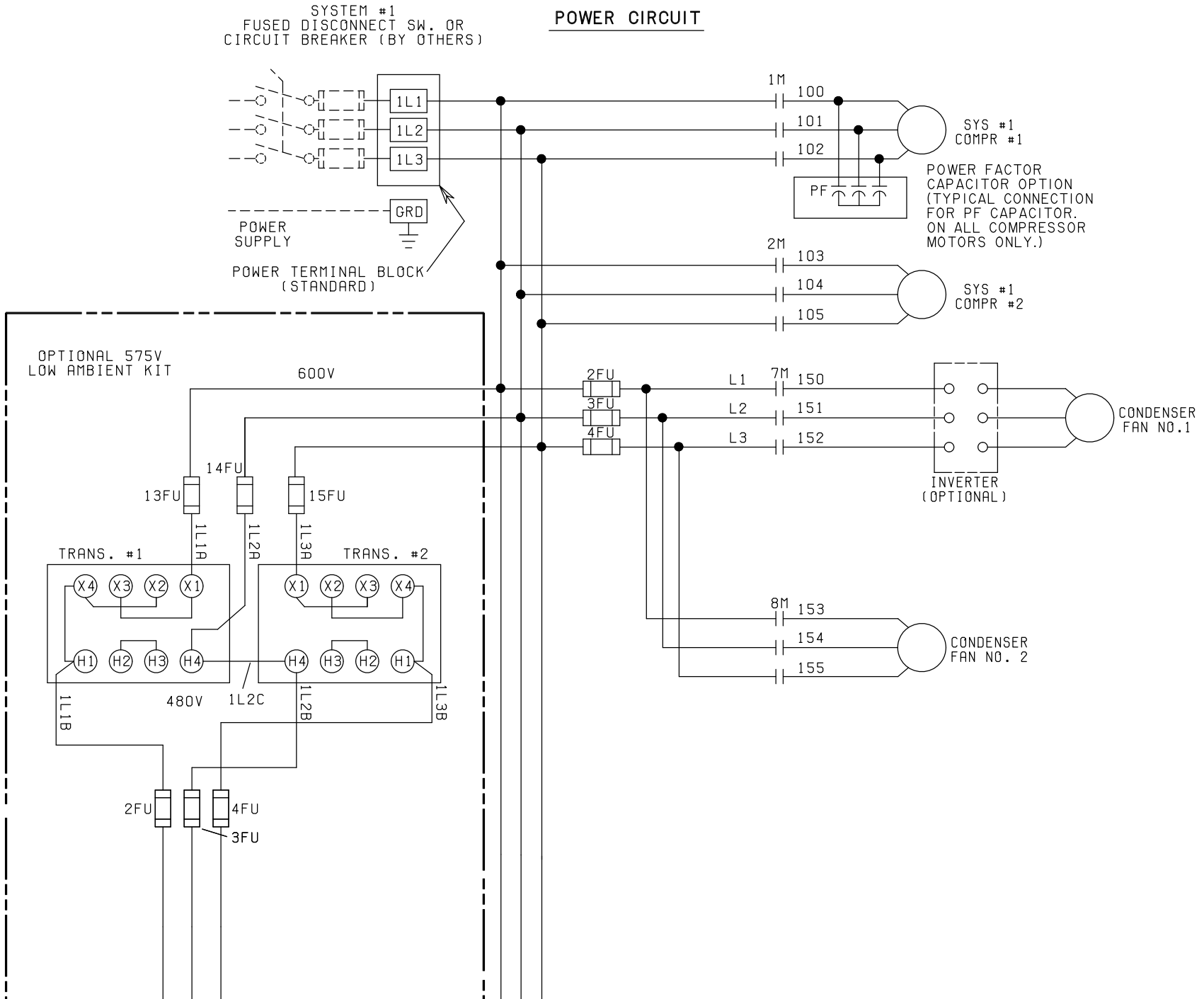
FIGURE 20 - POWER WIRING, SINGLE CIRCUIT
