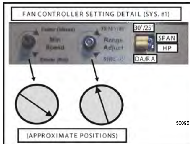
FIGURE 47 - POTENTIOMETER SETTINGS
