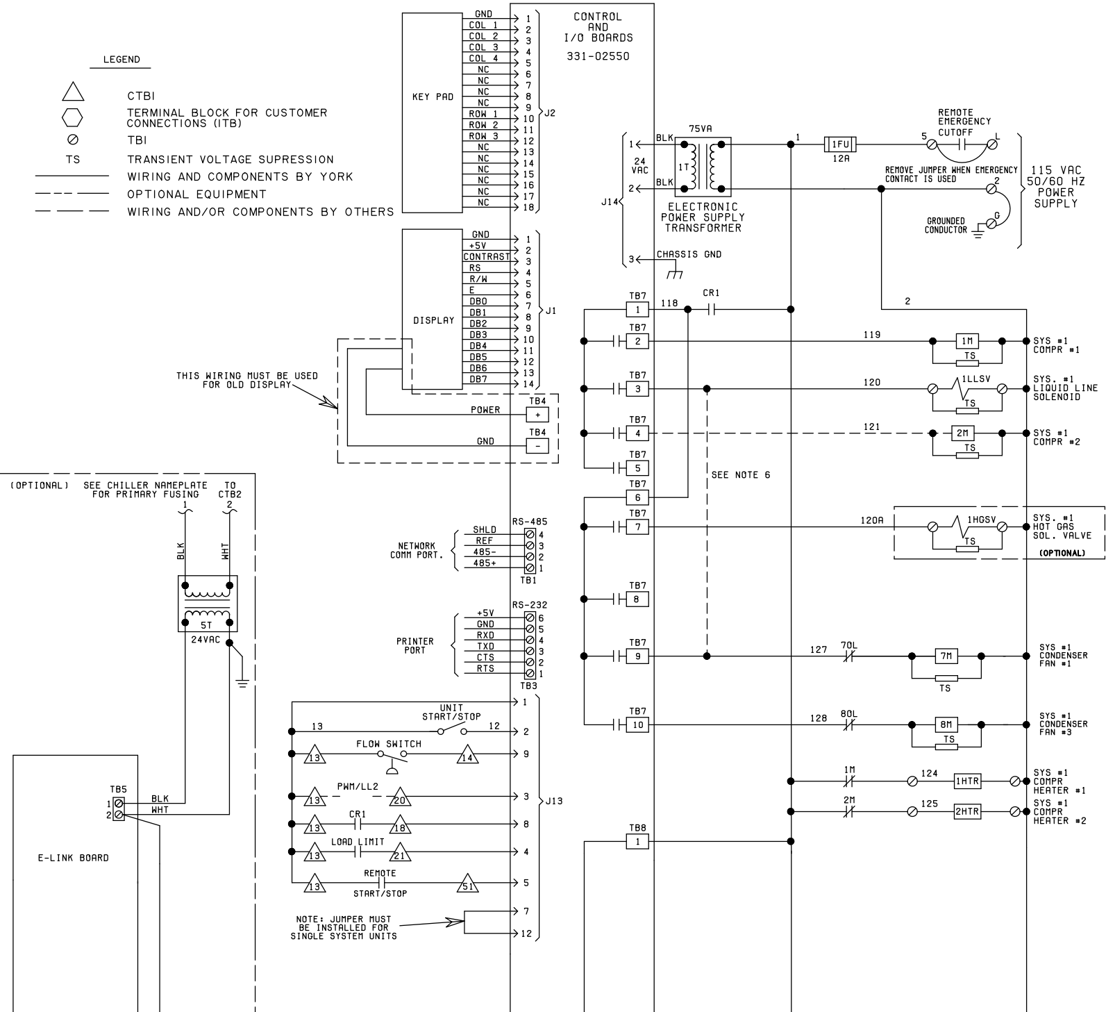
FIGURE 13 - CONTROL WIRING DIAGRAM, SINGLE CIRCUIT, IPU II
